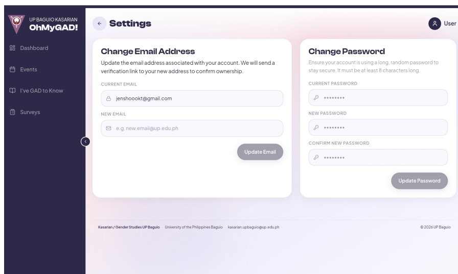
Figure 32: Settings Page
